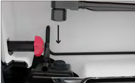
5.1 Connect the battery cable to the control box by pushing the plug into the socket.
